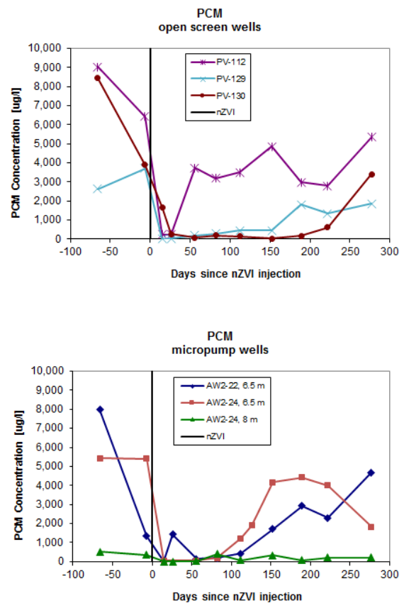
Figure 10. PCM concentrations in groundwater after NANOFER 255 injection.
