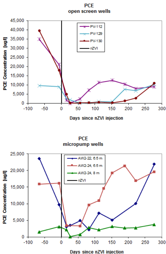
Figure 9. PCE concentrations in groundwater after NANOFER 255 injection.
