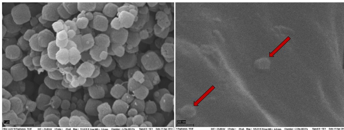
Figure 30 Scanning electron micrographs of (left picture) Fe zeolite on filter paper at the end of the germination test; (right picture) individual Fe zeolite particles strongly attached to a radish root (exposure concentration 1 g/L).
