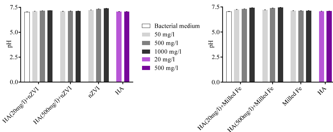
Figure 36 pH values of positive control nZVI (left) and milled Fe particles (right) suspended in bacterial growth medium, with and without humic acids (HA).
